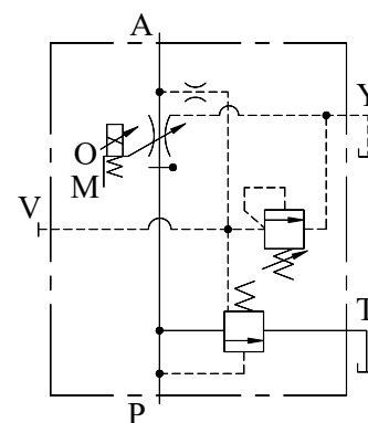
Without Proportional Pilot Relief Valve
